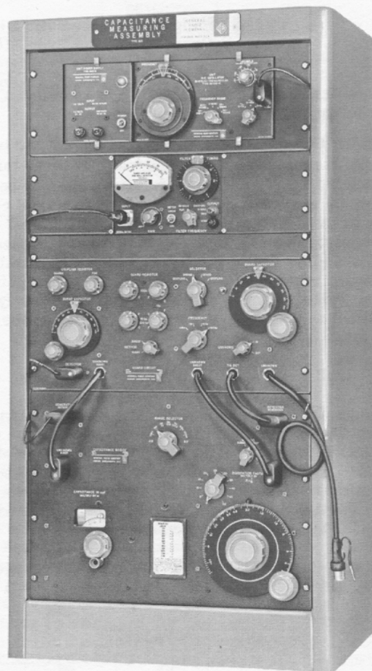
Figure 6. View of Type 1610-B Capacitance Measuring Assembly: Type 1210-C Unit R-C Oscillator with Type 1203-B Unit Power Supply, Type 1232-A Tuned Amplifier and Null Detector, Type 716-P4R Guard Circuit, and Type 716-CR Capacitance Bridge.
