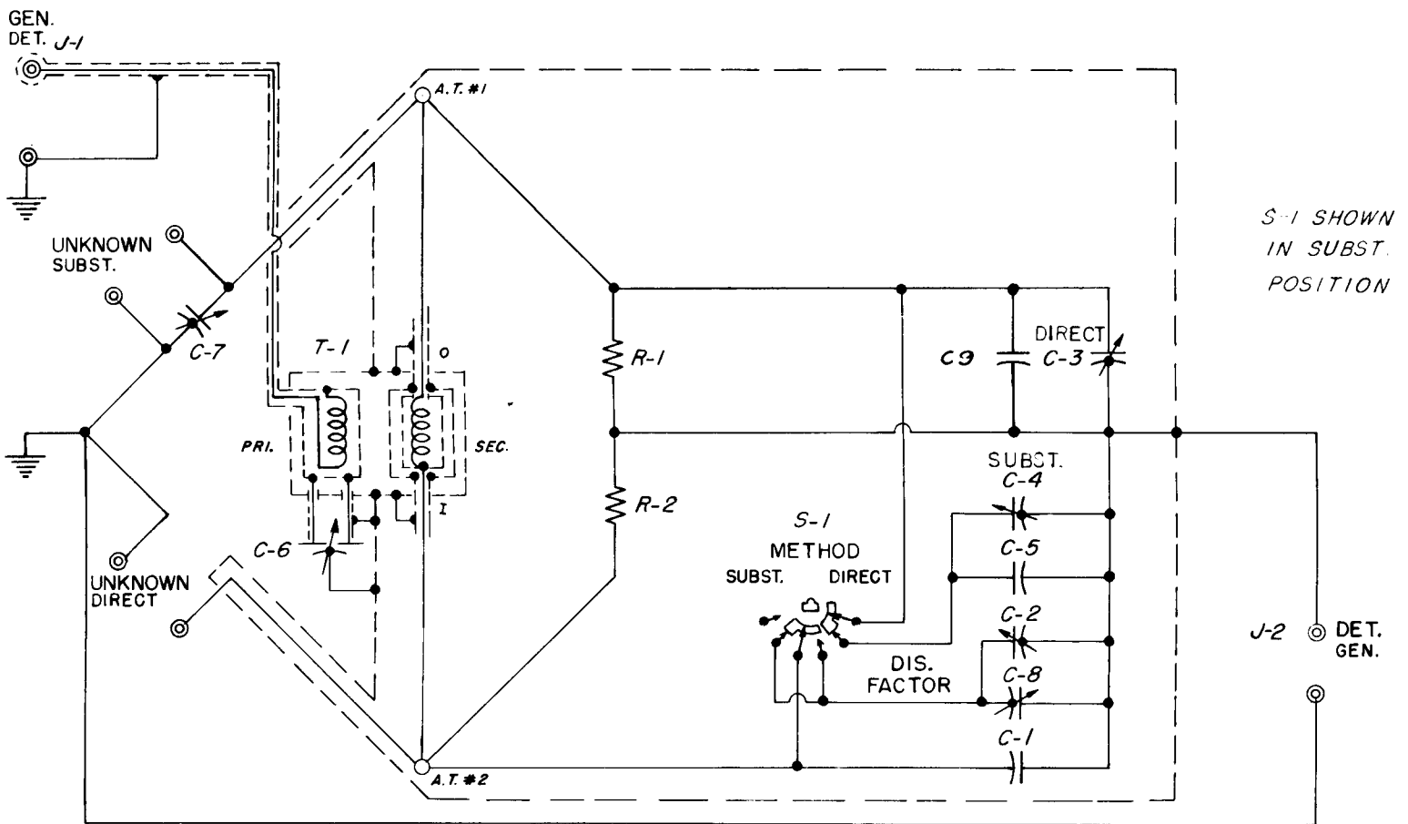
Wiring Diagram for Type 716-CS1 Capacitance Bridge
