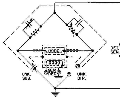
Figure 10. Wiring Diagram for Type 716-C Capacitance Bridge.
