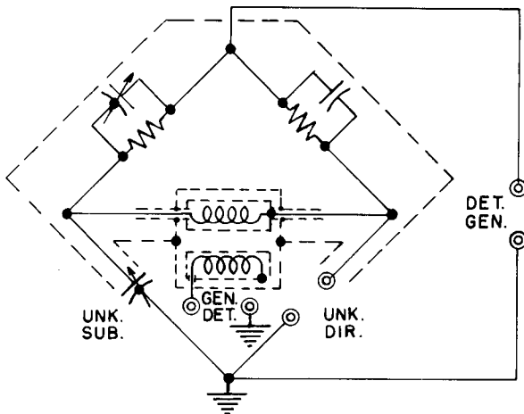
Elementary Schematic Diagram
